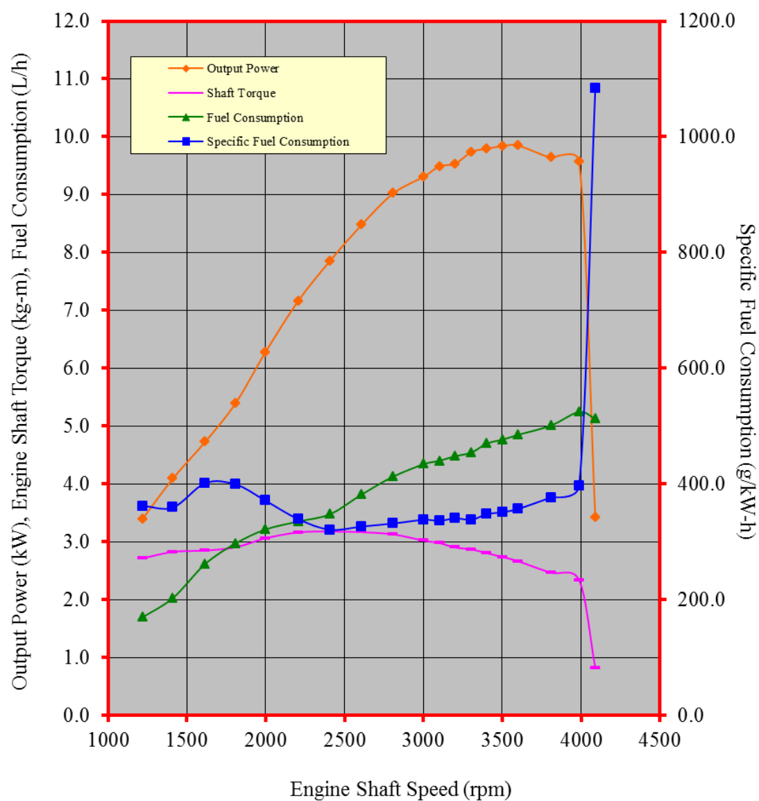
Figure 3. Performance characteristic curves of the HONDA GX390 MEGA MARINE gasoline engine
