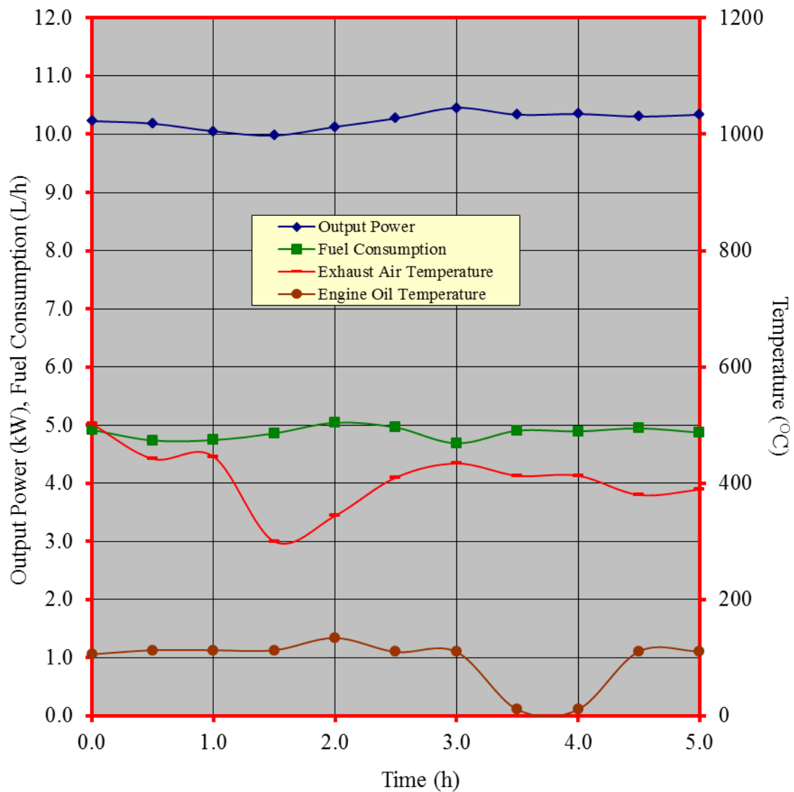
Figure 4. Performance characteristic curves during the continuous running test of the HONDA GX390 MEGA MARINE gasoline engine
